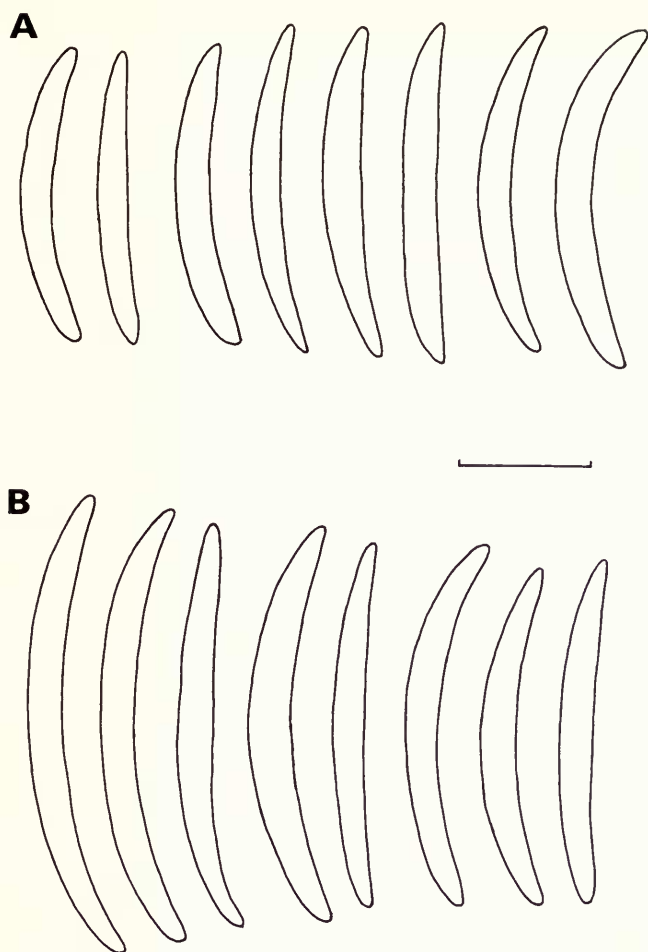
Fig. 43 Ascospore outlines (A) Cresporhaphis acerina (Rehm) Aguirre (W-isolectotype); (B) Cresporhaphis muelleri (Duby) Aguirre (W 3522/4155-holotype of Leptorhaphis aggregatus ); scale = 10 \mu m.
